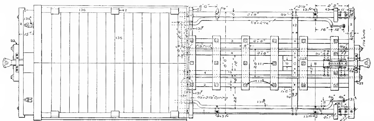
Fig. 329. Half Plan of Car and Half Plan of Underframe.
